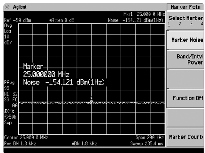
Figure 5. Marker noise function
