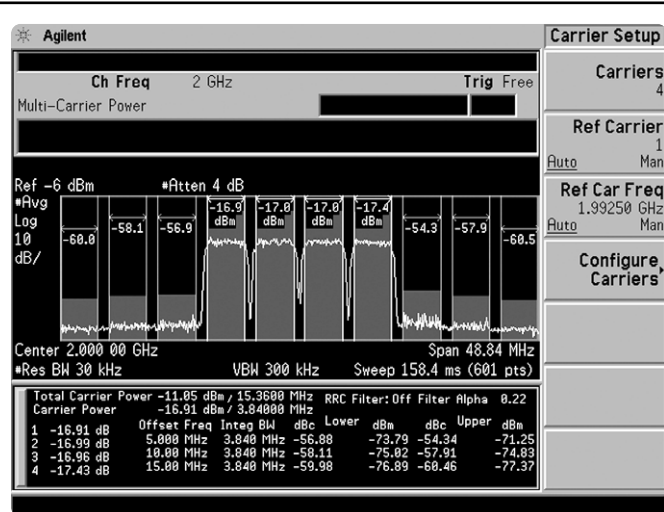
Figure 10. W-CDMA multi-carrier power measurement
