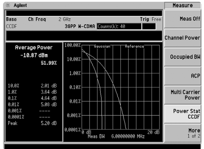
Figure 9. W-CDMA CCDF measurement
