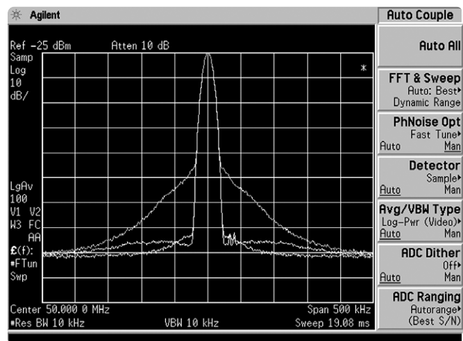
Figure 6. Phase noise optimization modes
