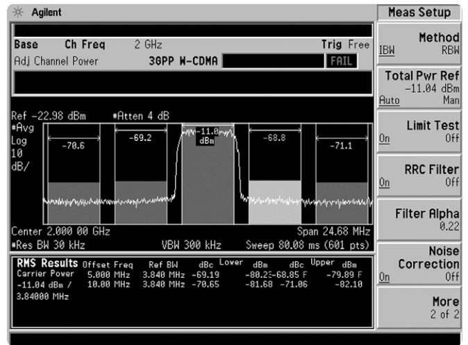
Figure 8. W-CDMA ACP measurement
