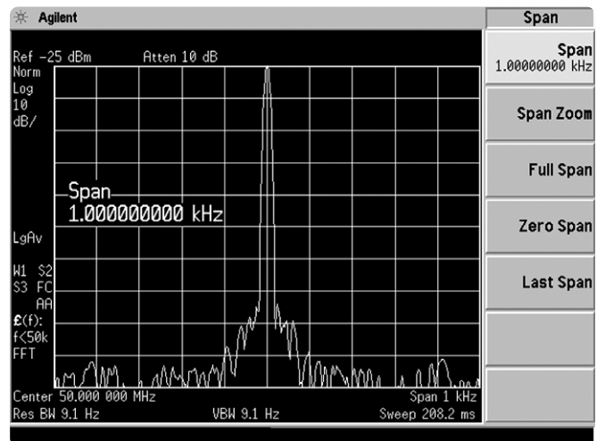
Figure 7. FFT mode operation
